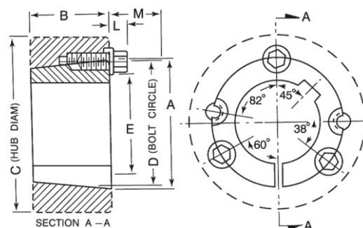
Structure for 6050
