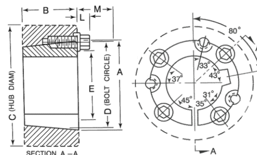
Structure for 7060 & 8065
